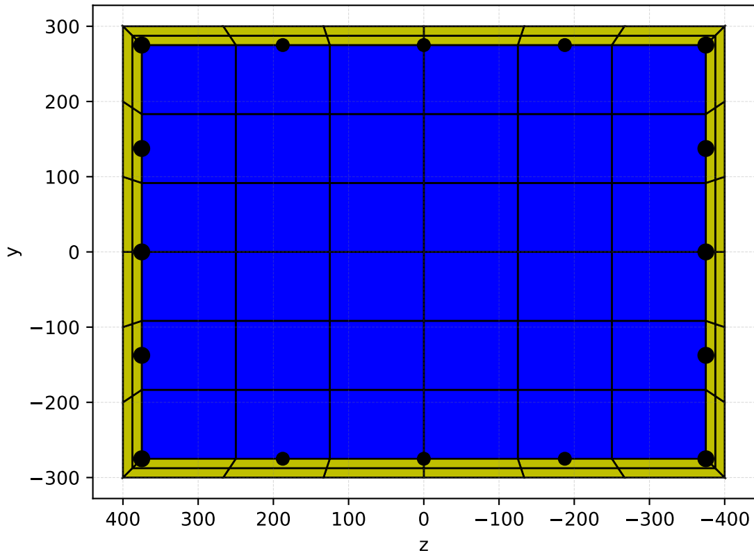
Beam Section for tank bottom
